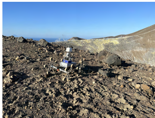
Figure 11: Asguard IV during field tests on the volcano crater at Vulcano Island.
