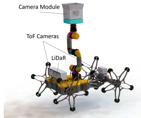
Figure 5: Placement of camera module (Fig. 4) and additional sensors on Coyote III.
